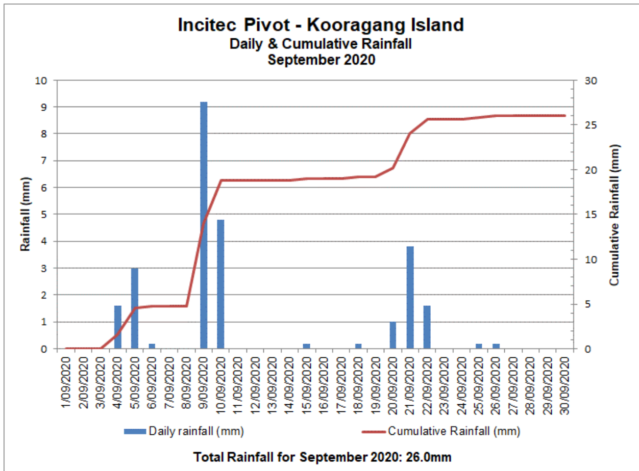
Figure 1 September 2020 Rainfall Summary
